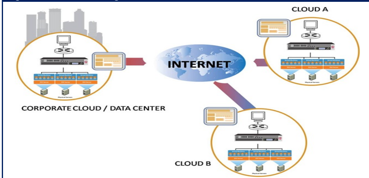
Figure 4: Cloud Balancing
