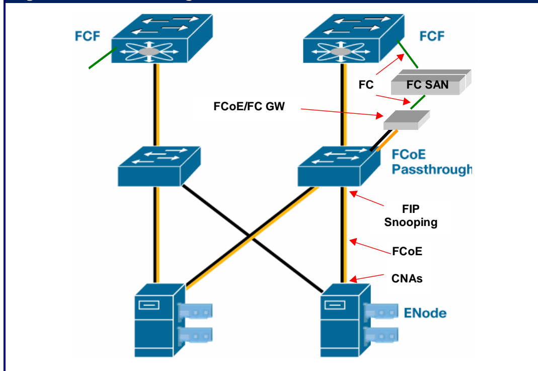
Figure 14: FCoE Converged LAN
