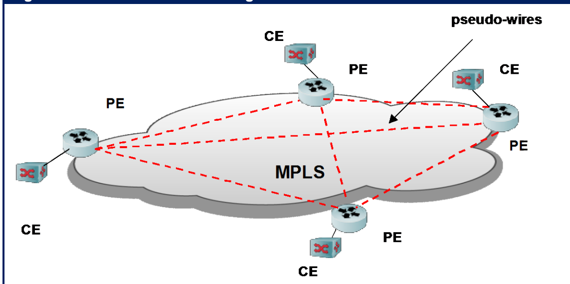
Figure 29: A VPLS Service Linking Four Customer Sites
